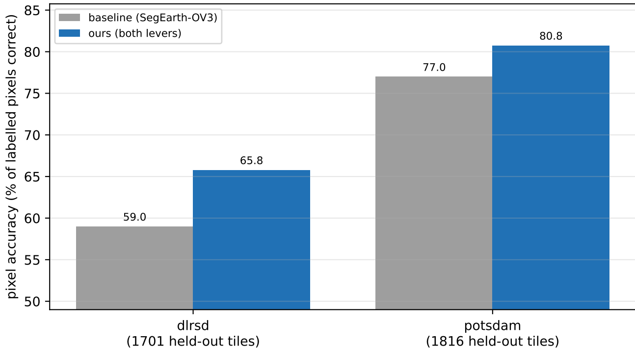
Overall pixel accuracy
