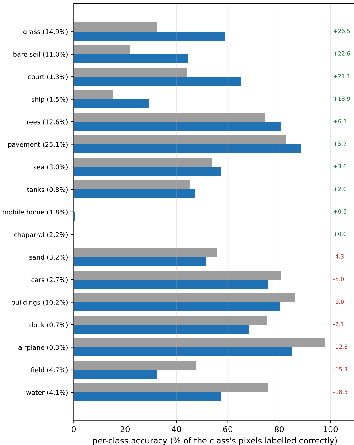
dlrsd — per class (right: change from baseline to ours; brackets: share of pixels)
