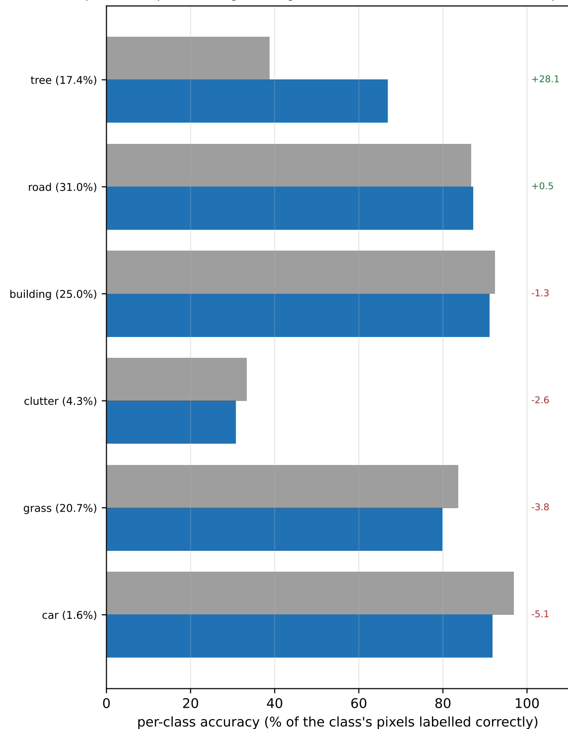
potsdam — per class (right: change from baseline to ours; brackets: share of pixels)
