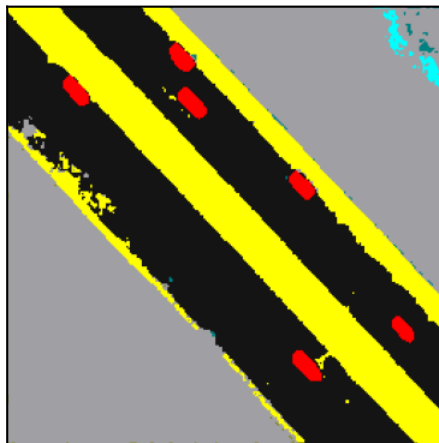
baseline \tau=0.1 19.3
