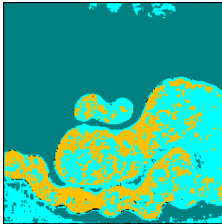
baseline \tau=0.1 30.2
