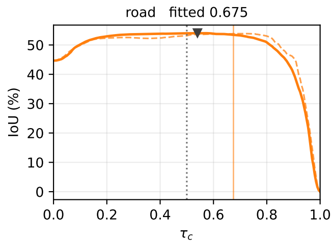
Per-class IoU against its own threshold, other thresholds held at the fitted vector
