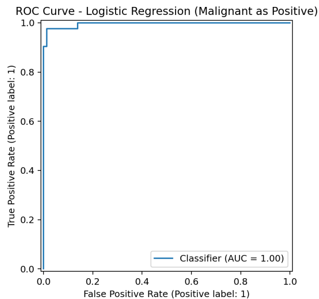
Figure 11: ROC curve for the final model, treating malignant as the positive class.
