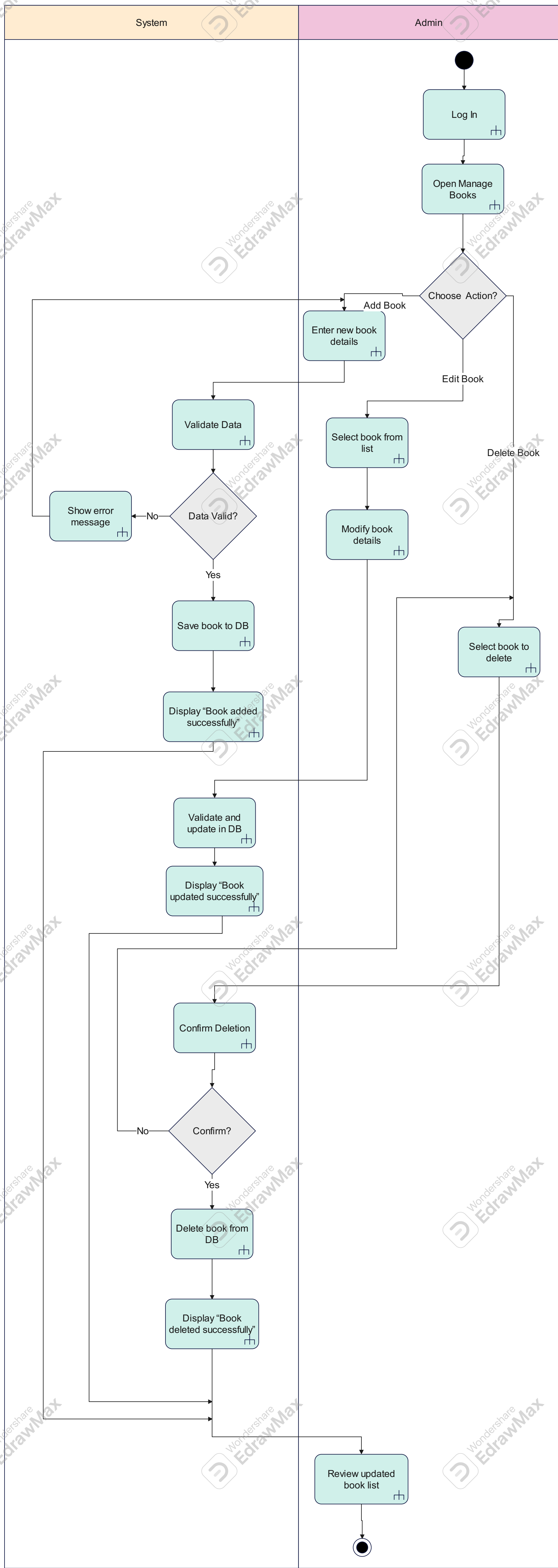
Activity Diagram: "Manage Books"
