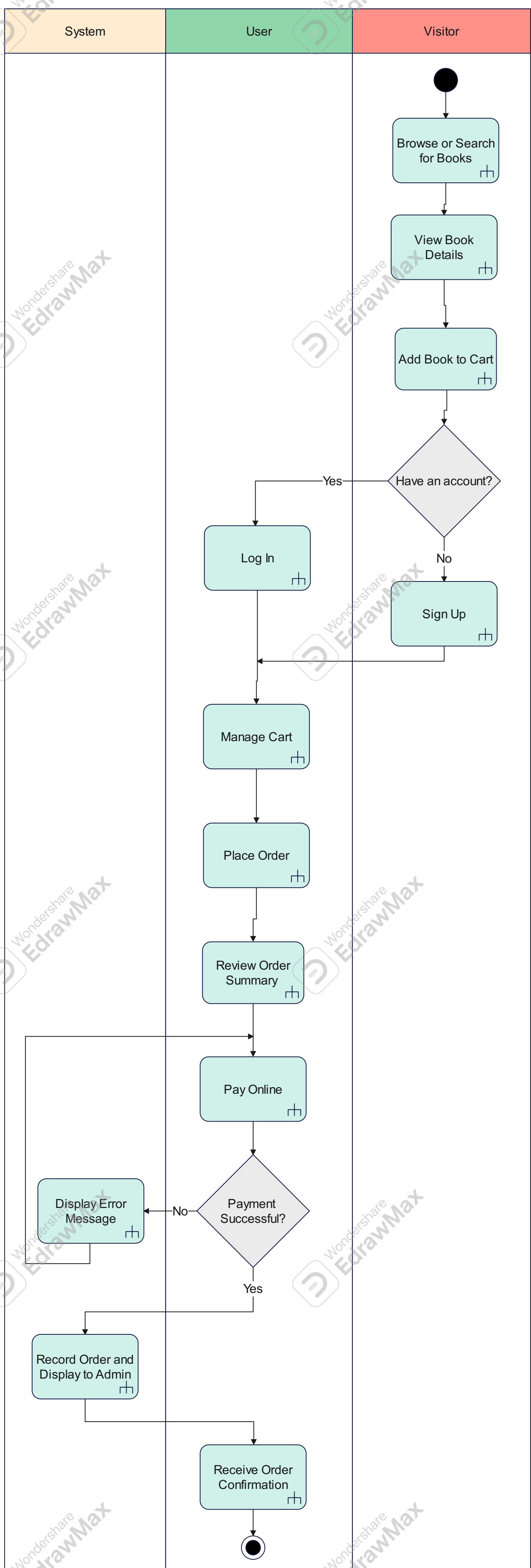
Activity Diagram: "Place Order"
