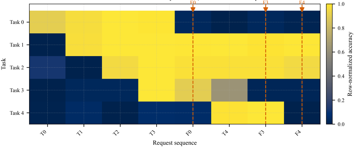
Row-normalized Per-task Accuracy Timeline | CIFAR-10 PALL-Adapter
