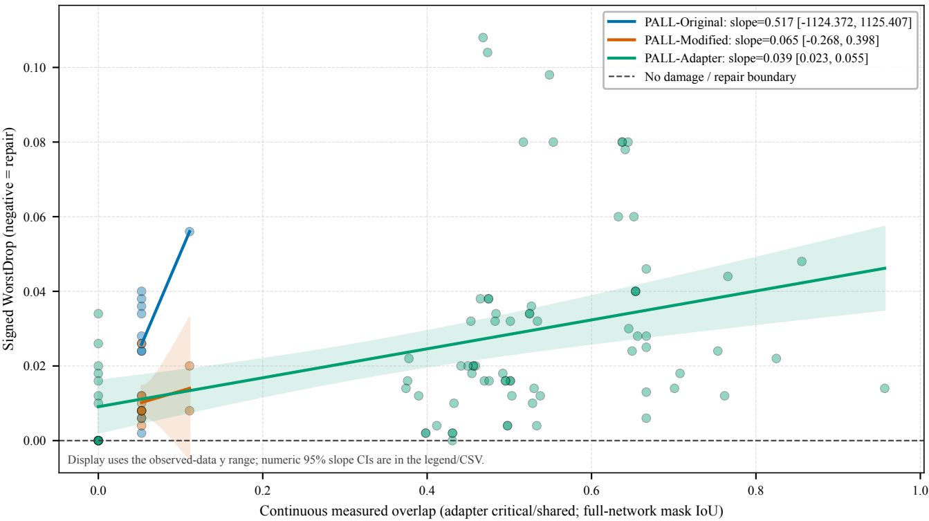
CIFAR-100 overlap response (primary; pooled completed runs)
