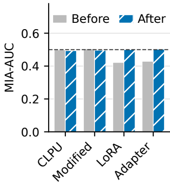
CIFAR-10
