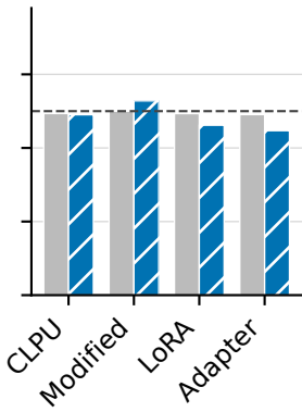
CIFAR-100
