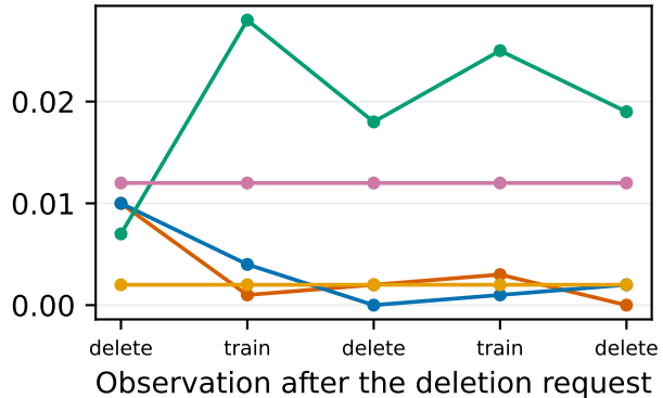
CIFAR-100
