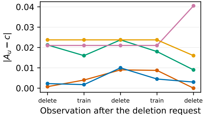
CIFAR-10
