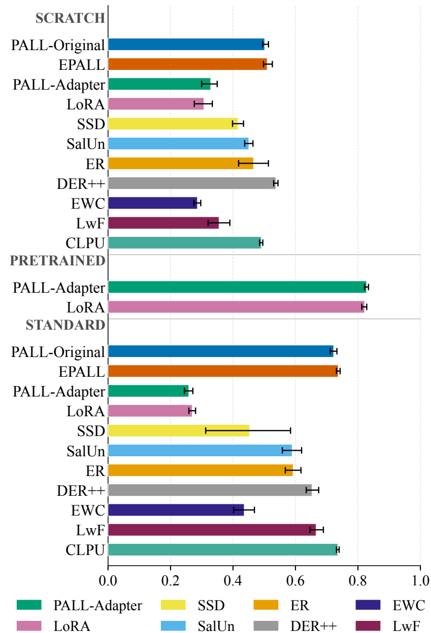
(b) CIFAR-100
