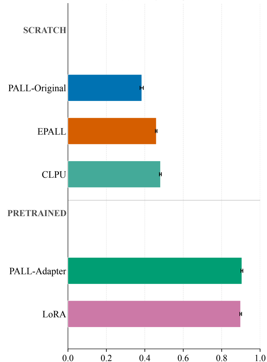
(c) TinyImageNet
