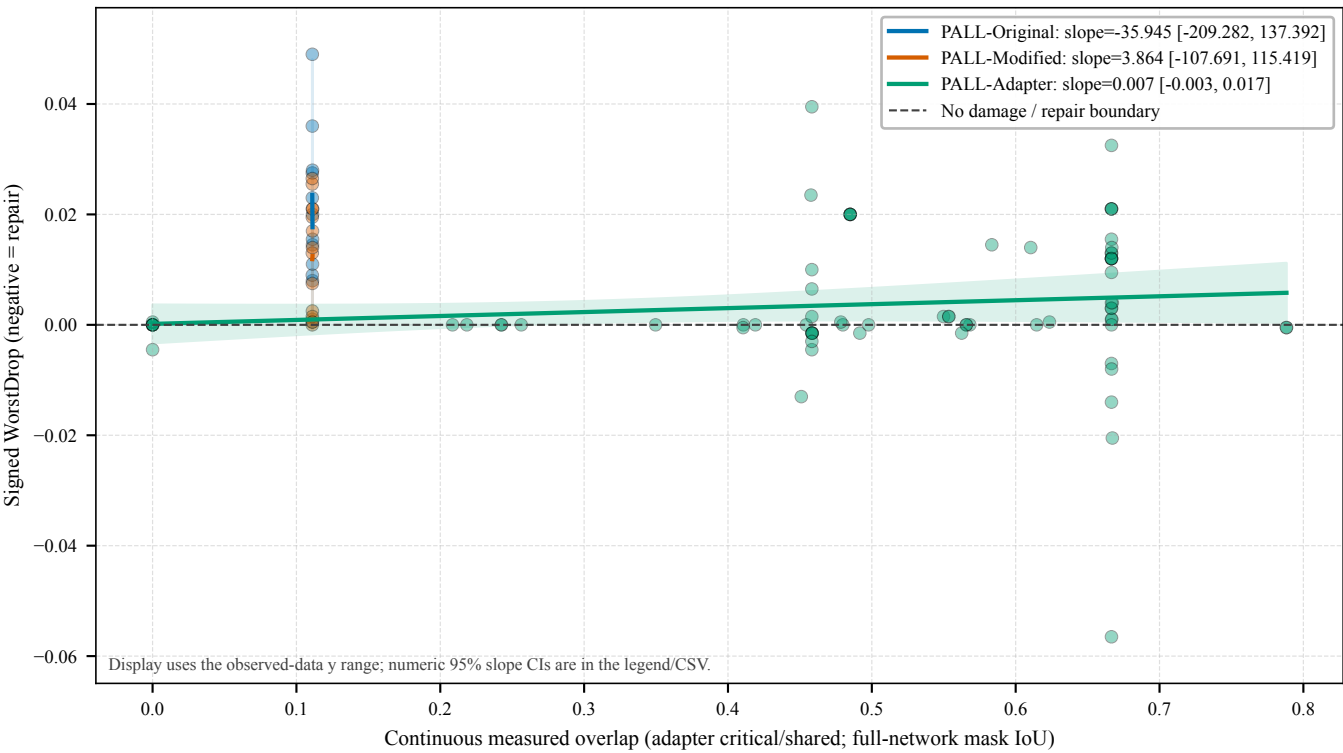
CIFAR-10 overlap response (secondary; pooled completed runs)
