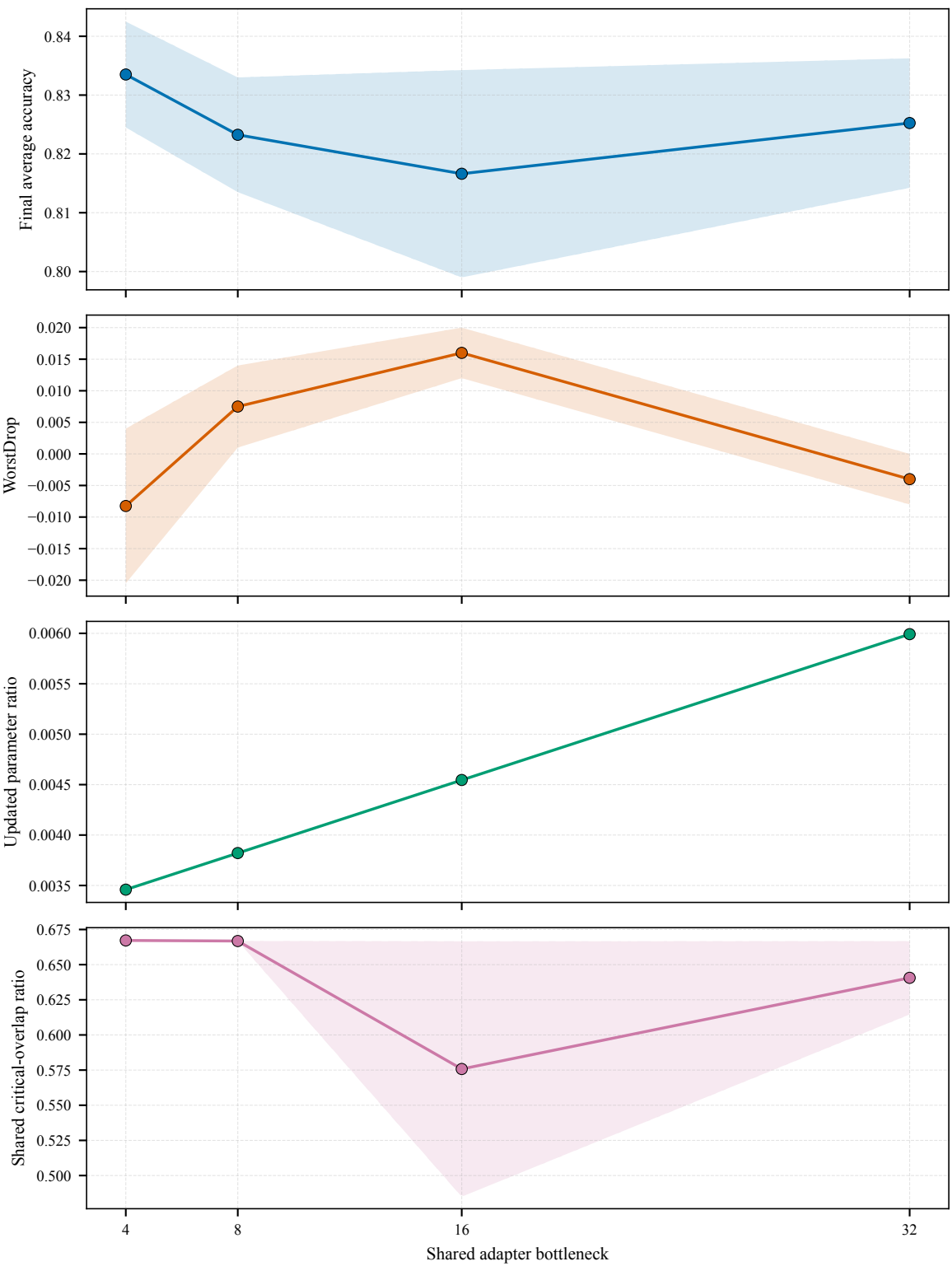
PALL-Adapter Shared-Bottleneck Ablation (CIFAR-10) | 95% bootstrap CI bands
