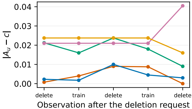
CIFAR-10
