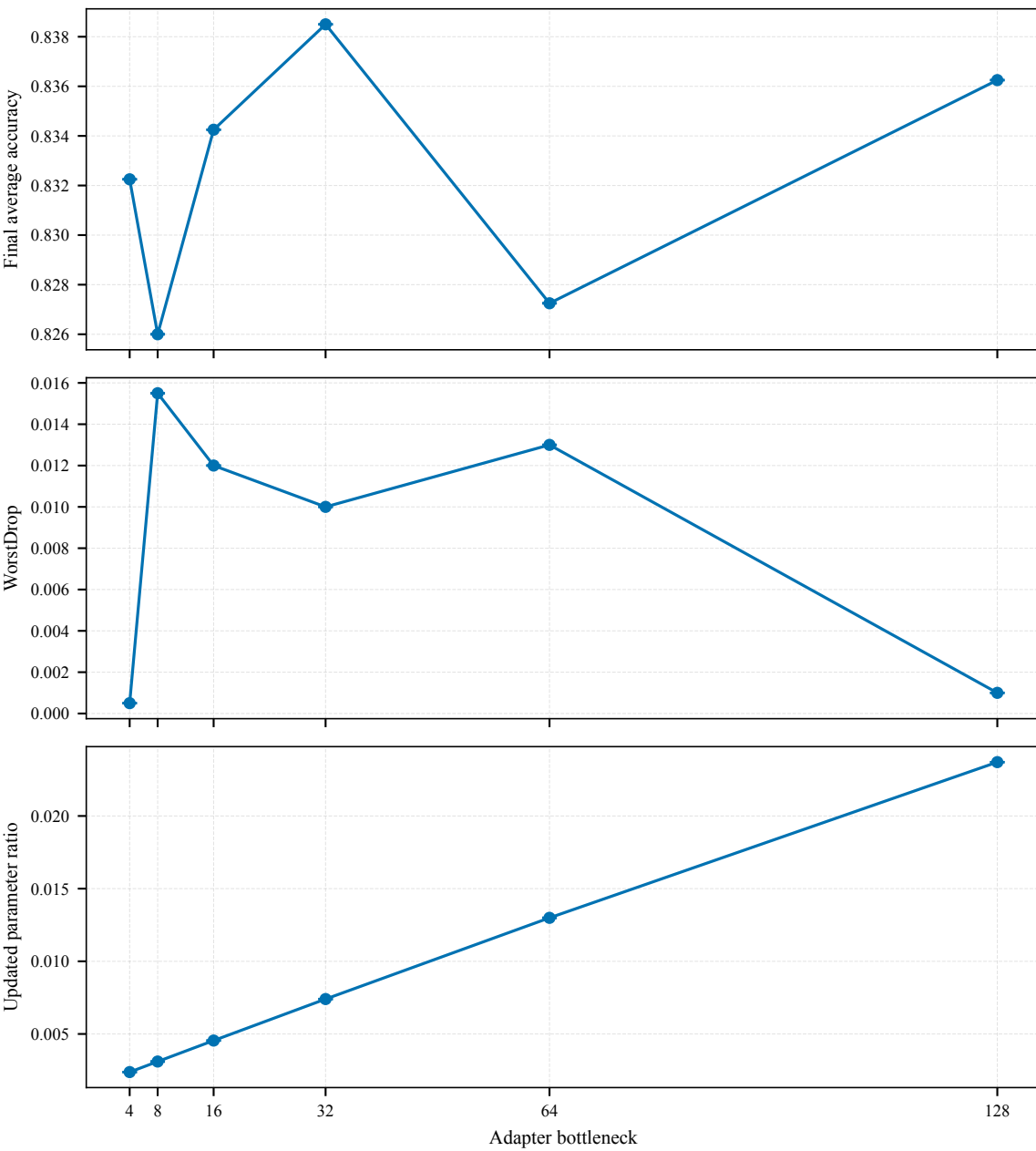
PALL-Adapter Bottleneck Ablation (CIFAR-10)
