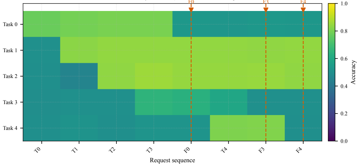
Per-task Accuracy Timeline | CIFAR-10 PALL-Adapter
