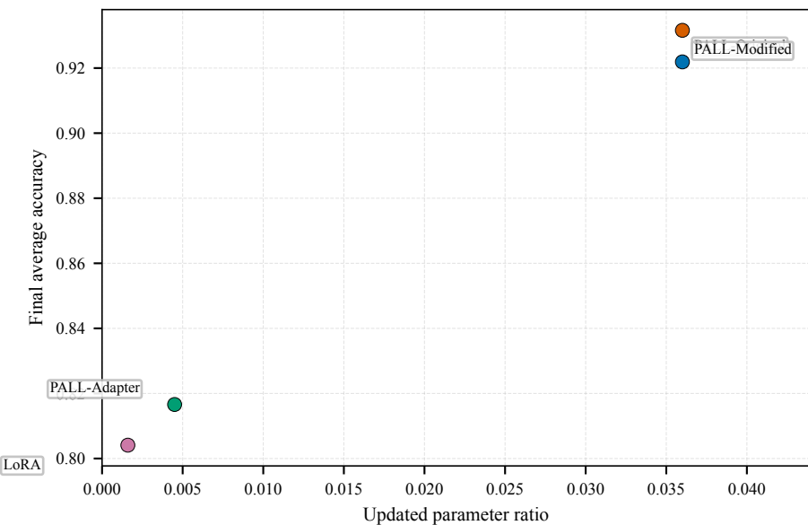
CIFAR-10 | From scratch
