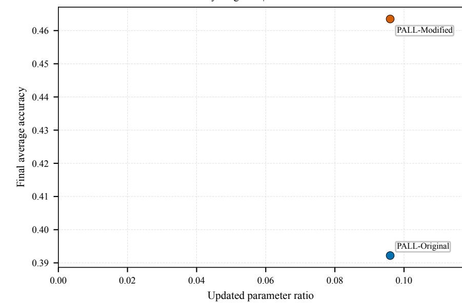
TinyImageNet | From scratch
