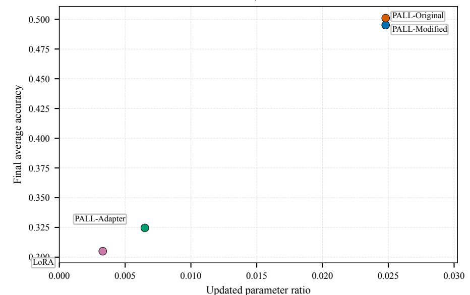
CIFAR-100 | From scratch
