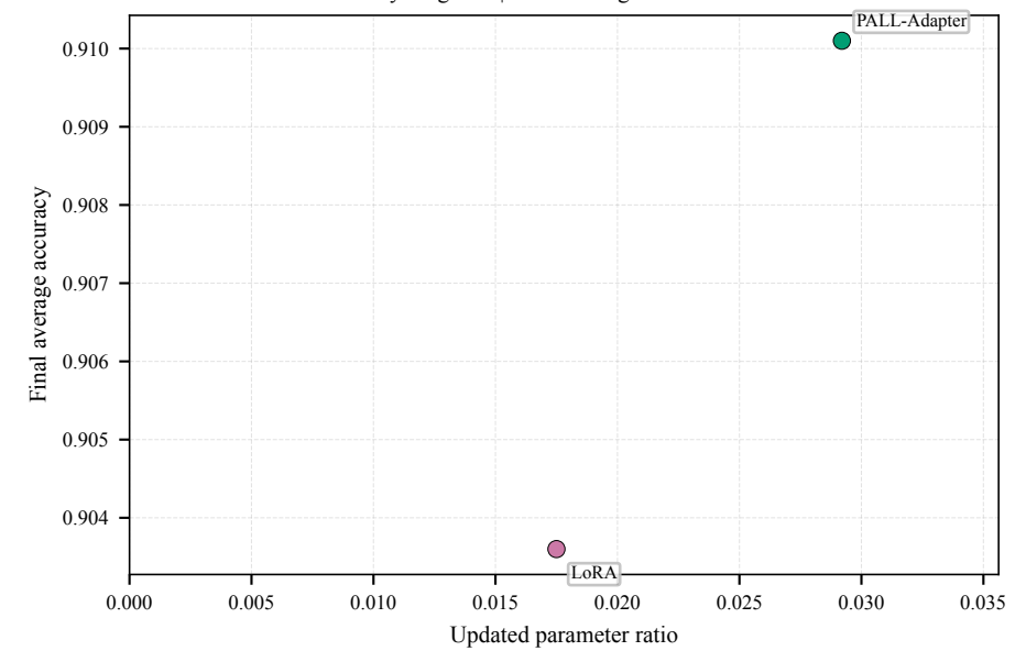
TinyImageNet | Frozen ImageNet backbone
