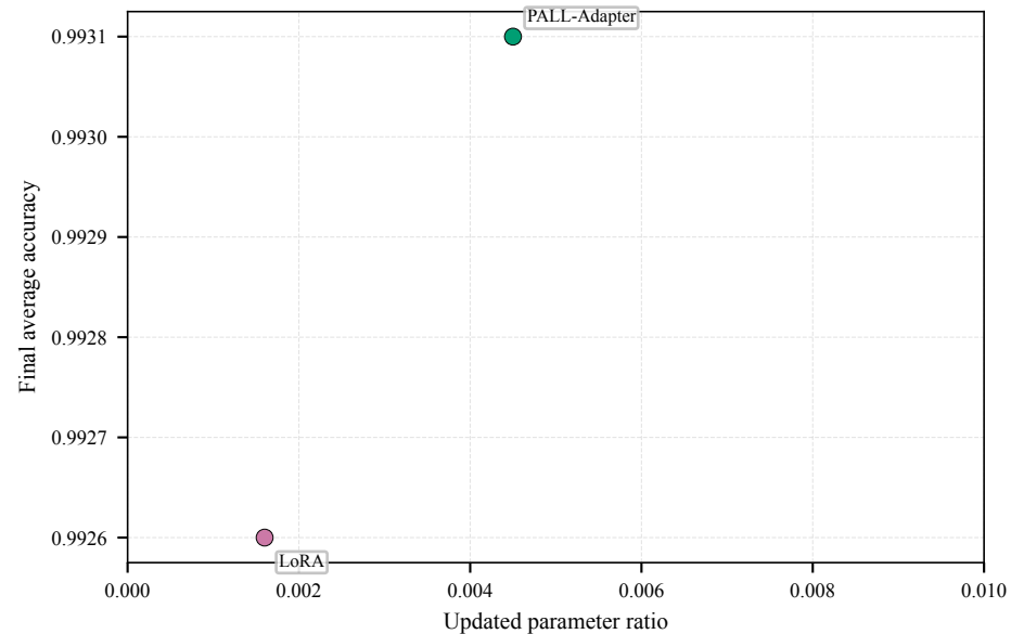
CIFAR-10 | Frozen ImageNet backbone
