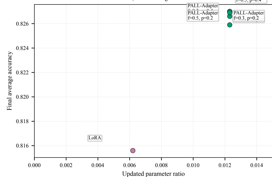
CIFAR-100 | Frozen ImageNet backbone
