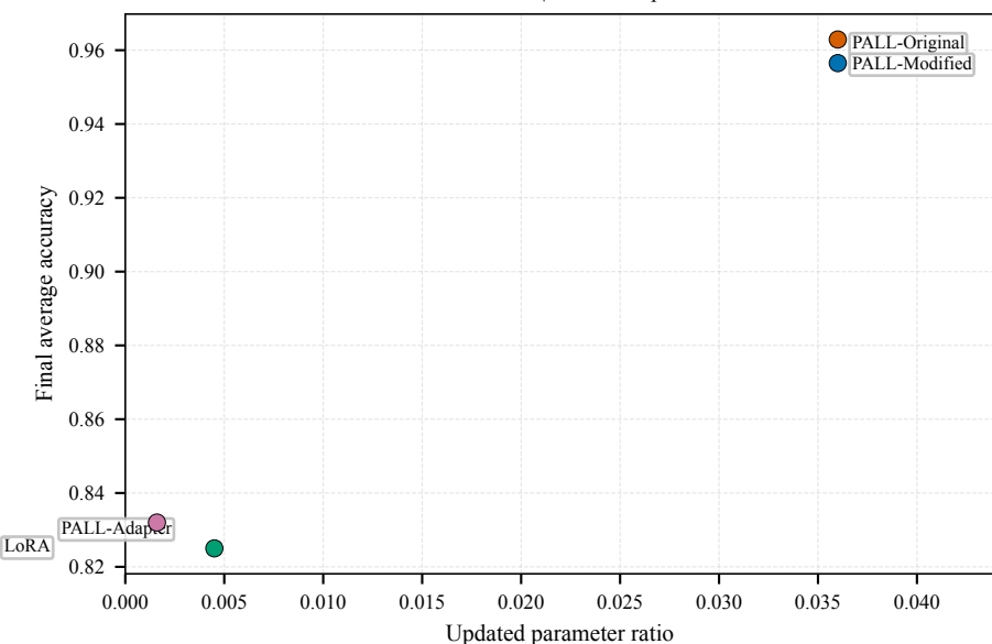
CIFAR-10 | Standard split
