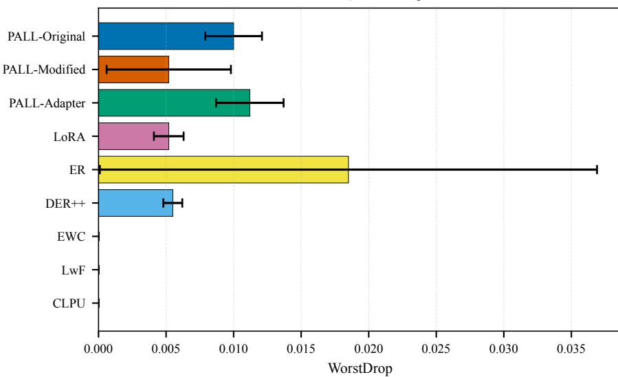
CIFAR-100 | Frozen ImageNet backbone
