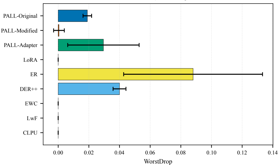
TinyImageNet | Frozen ImageNet backbone
