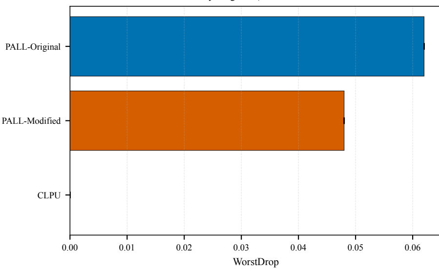
TinyImageNet | From scratch
