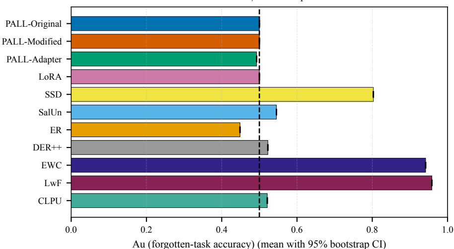
CIFAR-100 | Pretrained frozen
