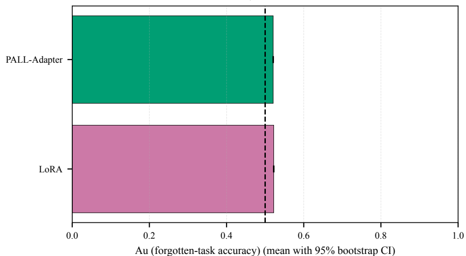
CIFAR-100 | From scratch
