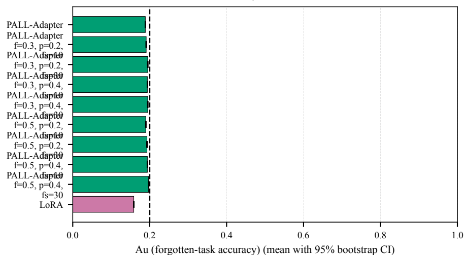
TinyImageNet | From scratch
