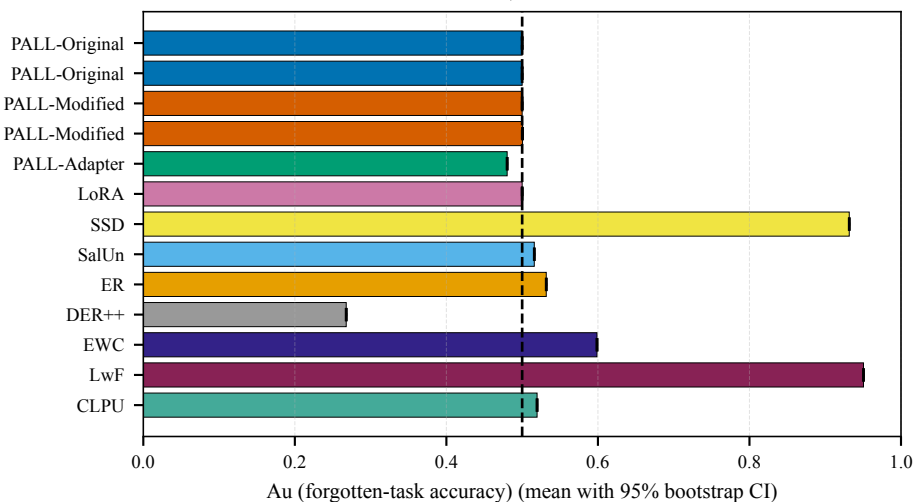
CIFAR-10 | Standard split
