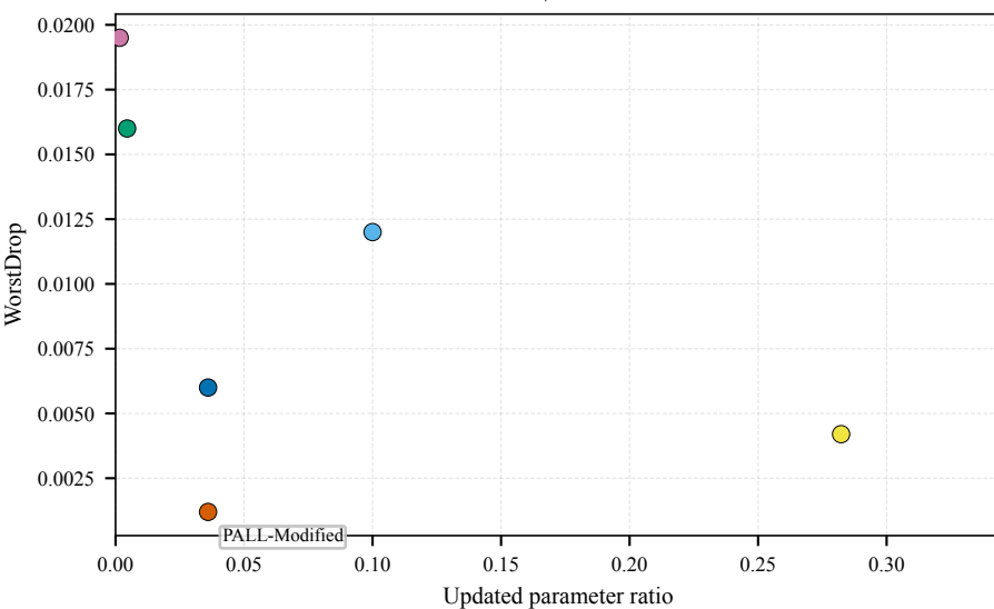
CIFAR-10 | Standard split
