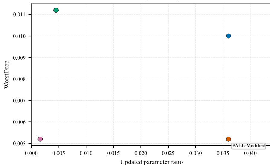
CIFAR-100 | Pretrained frozen
