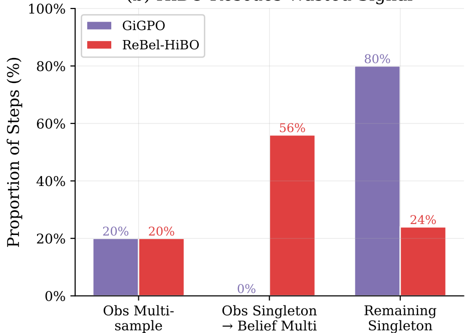
(b) HiBO Rescues Wasted Signal
