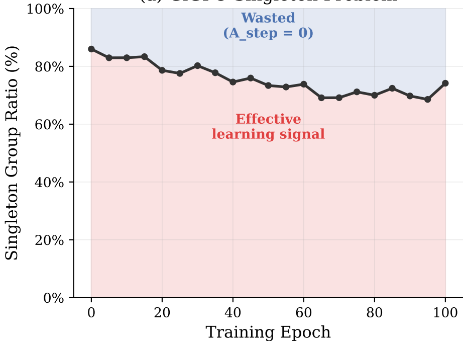
(a) GiGPO Singleton Problem
