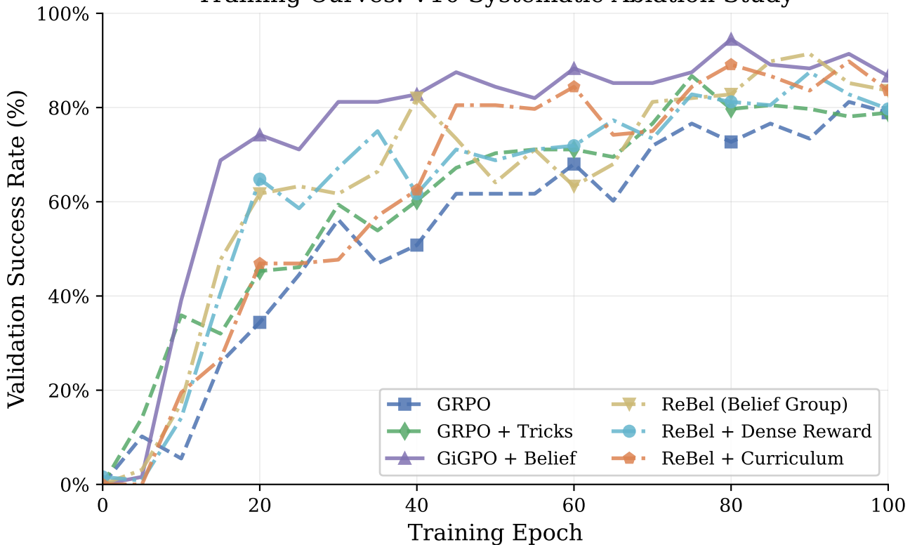
Training Curves: V10 Systematic Ablation Study
