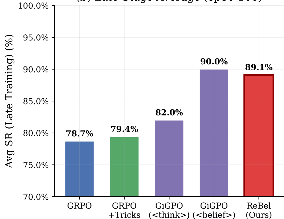
(b) Late-Stage Average (ep80-100)
