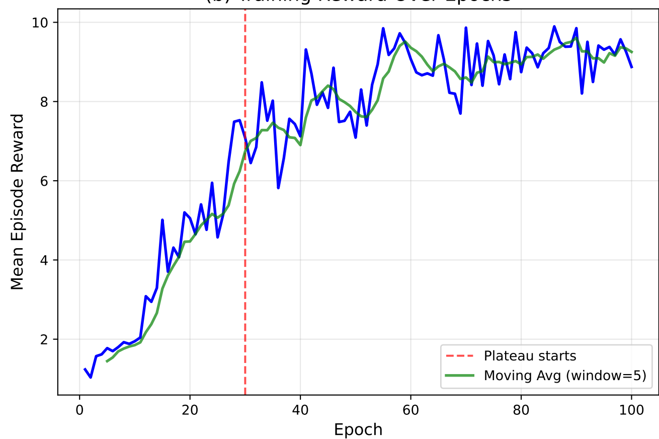
(b) Training Reward Over Epochs
