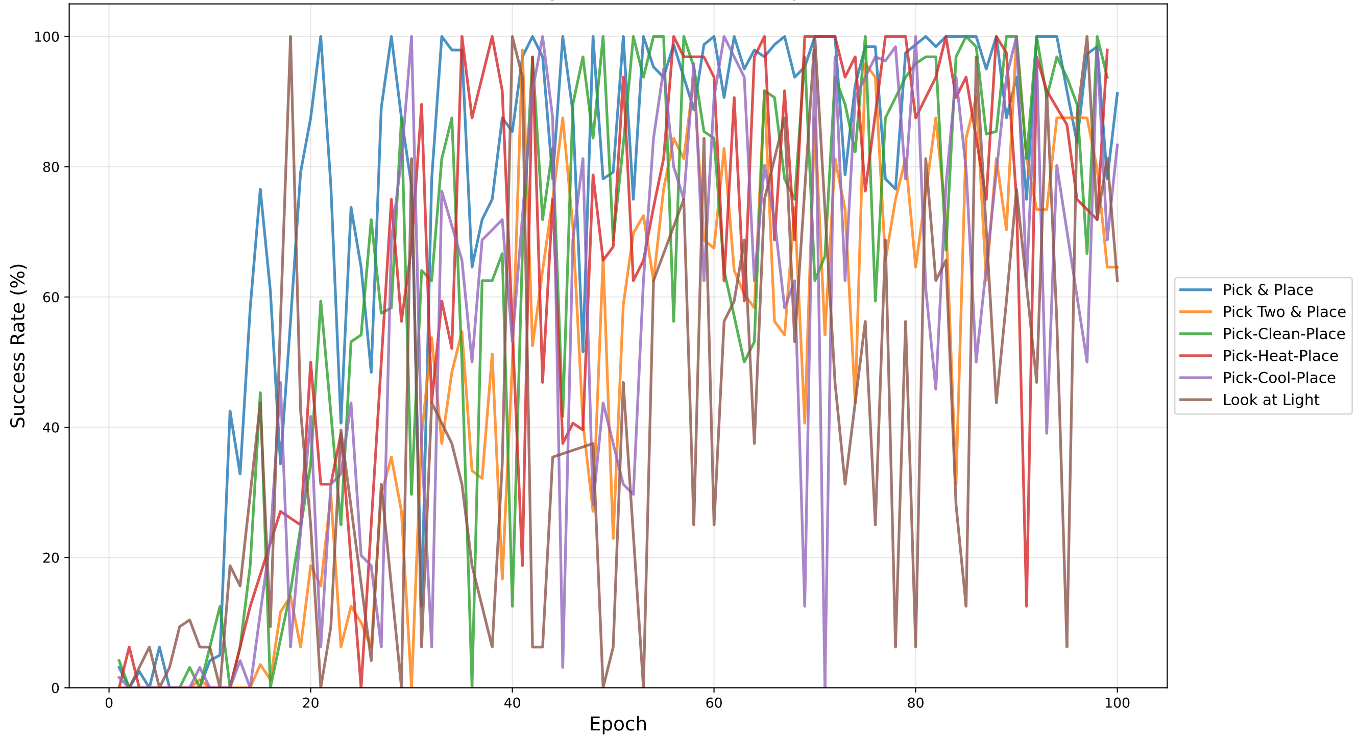
Per-Task Training Success Rate Over Epochs
