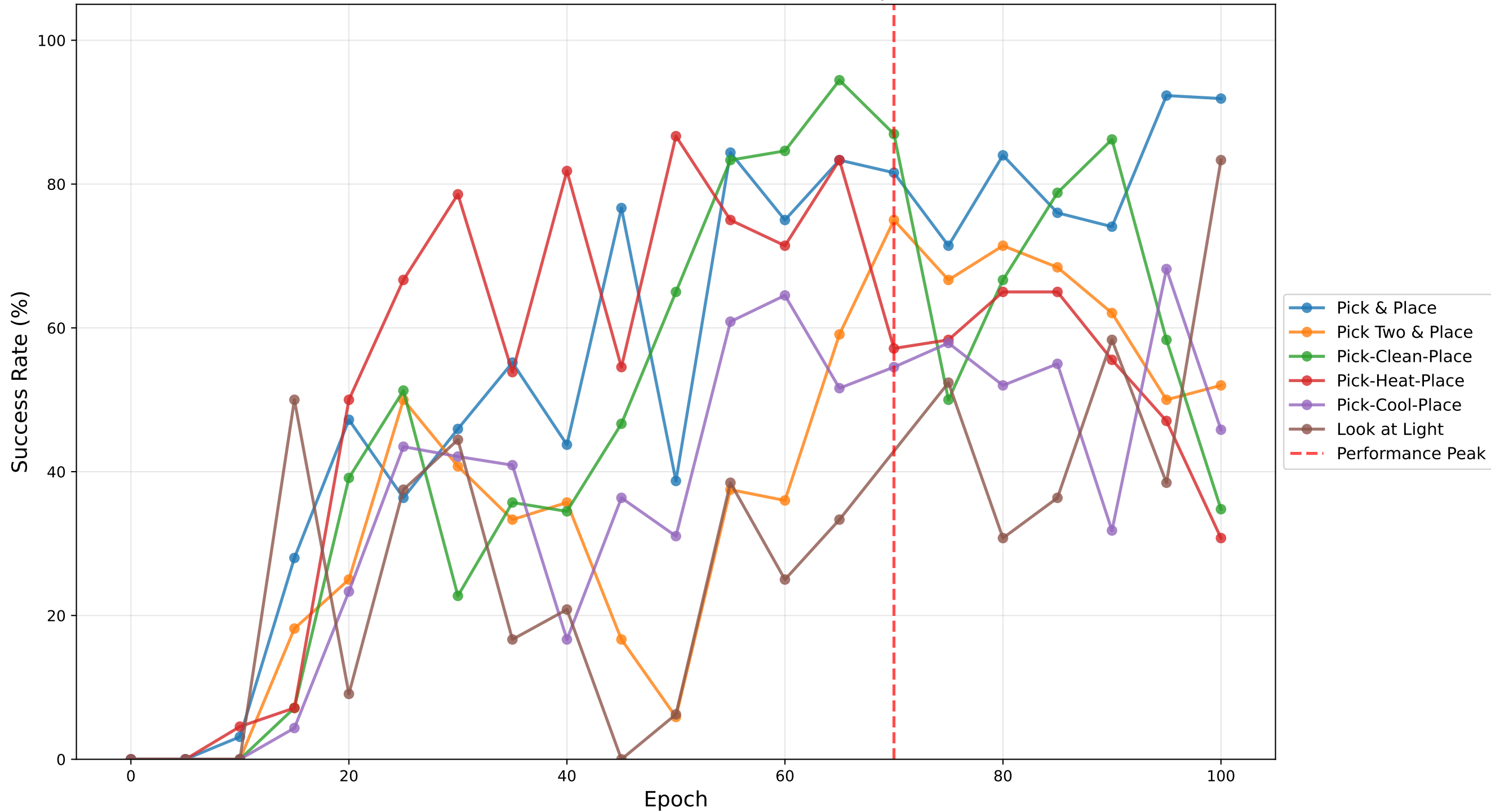
Per-Task Validation Success Rate Over Epochs
