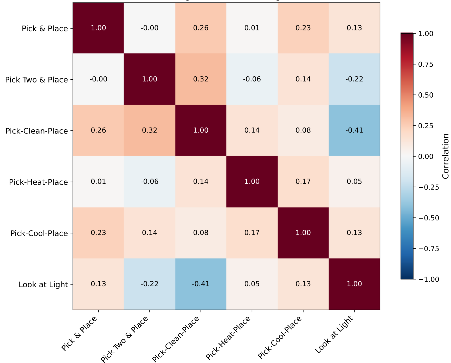
Task Improvement Correlation Matrix (Negative = Conflicting)
