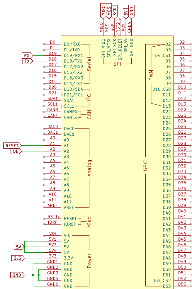
A1 Arduino_Due_Shield
