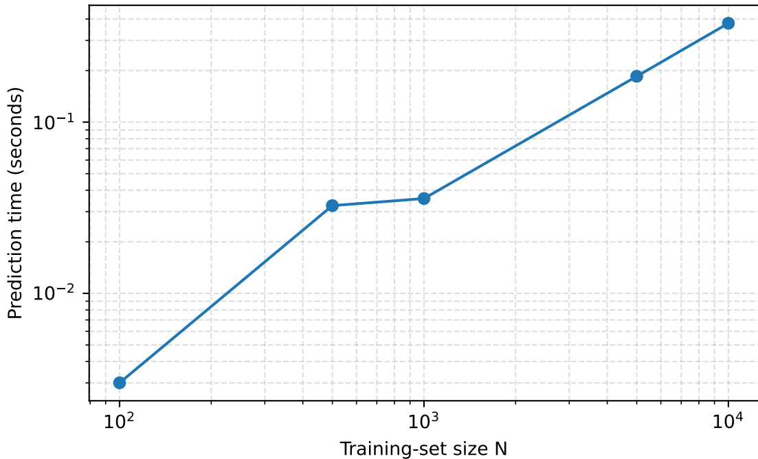
KNN Prediction Time vs N (empirical exponent 1.01)
