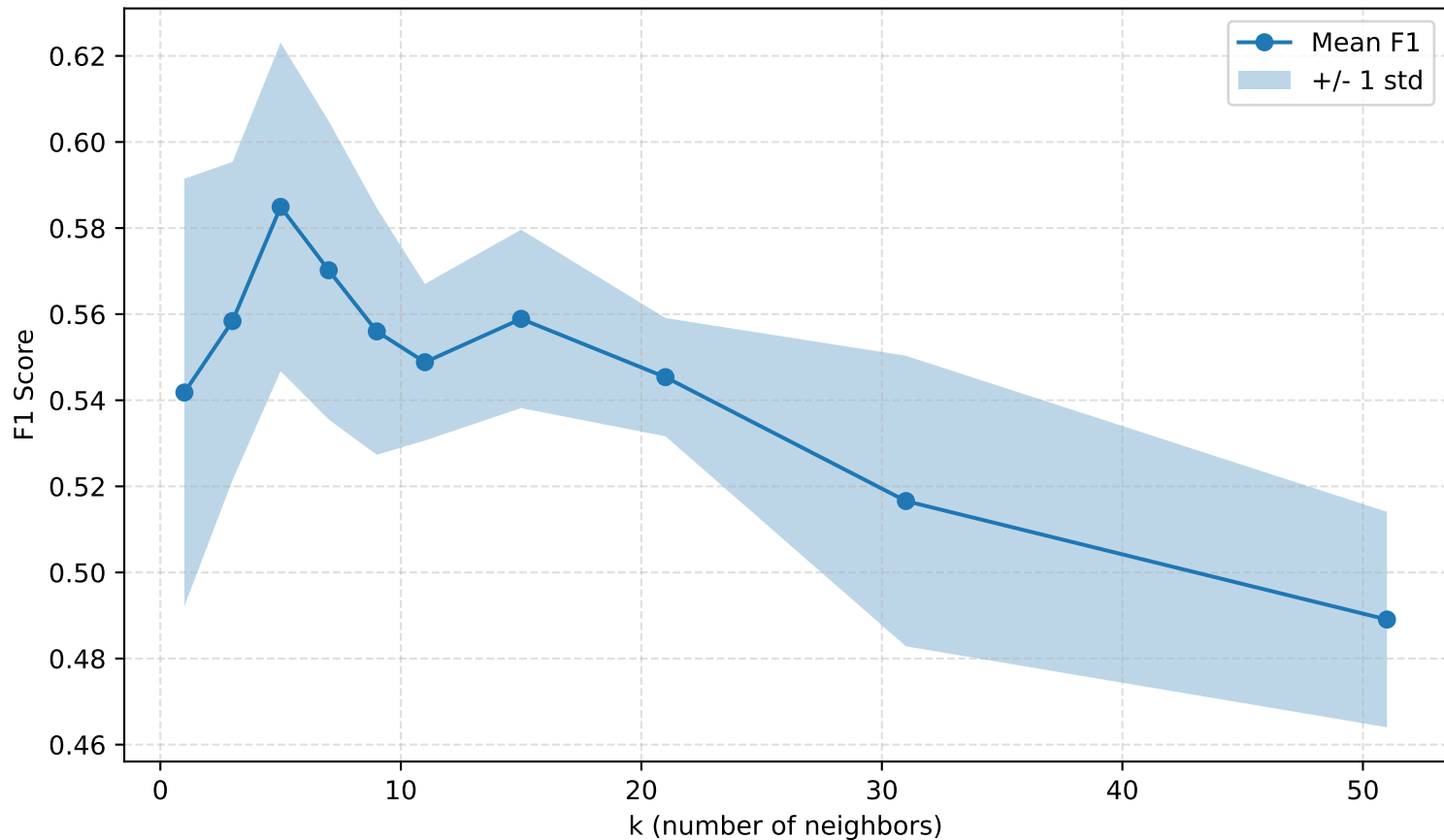
5-Fold Stratified CV - Mean F1 vs k
