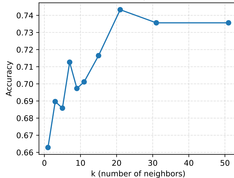
accuracy vs k
