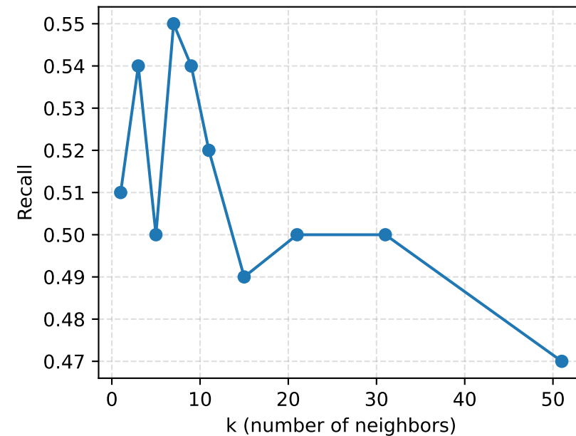
recall vs k
