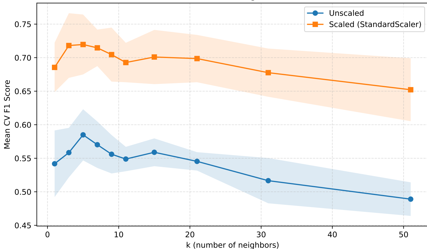
Effect of Feature Scaling on CV F1 vs k
