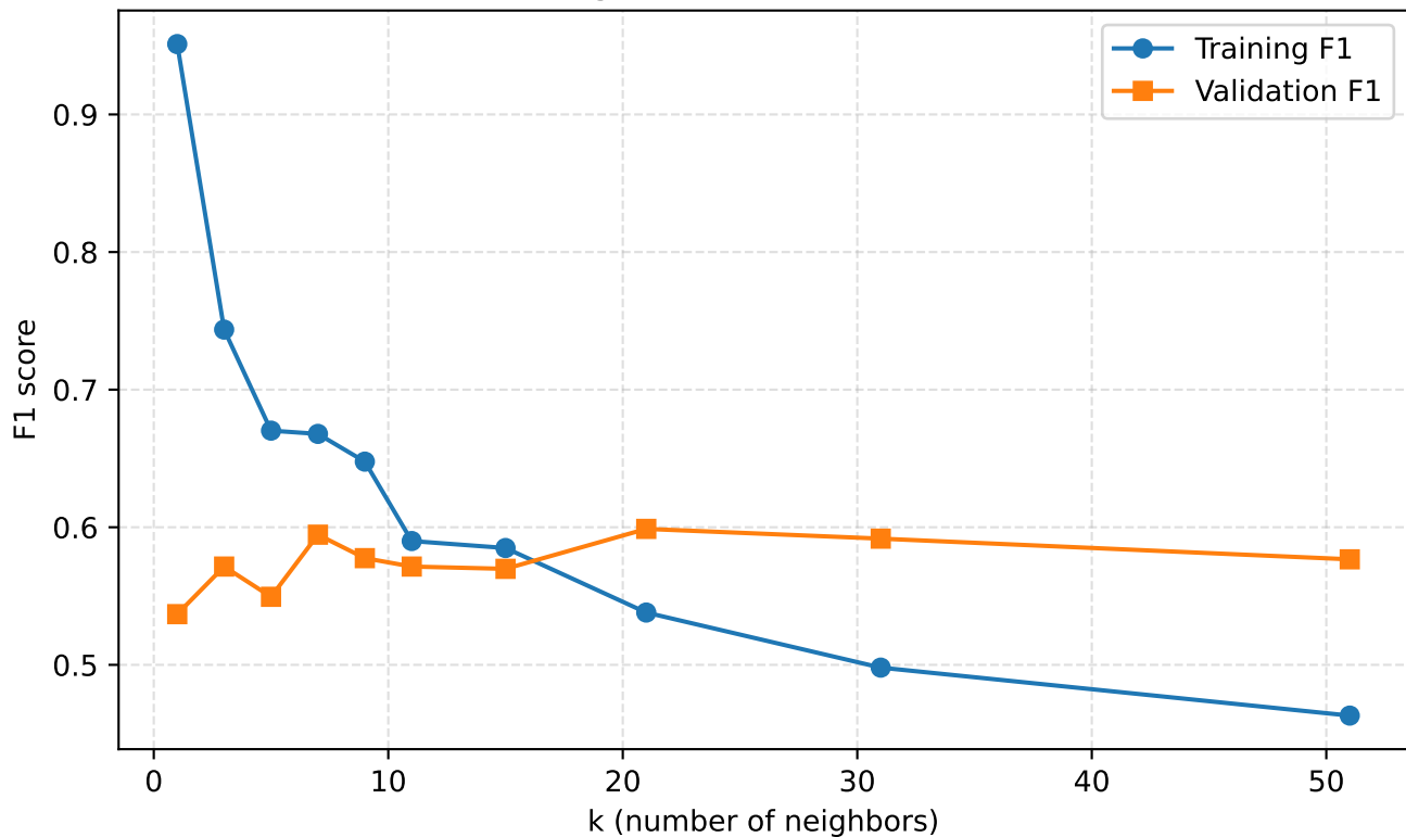
Training vs Validation F1 across k
