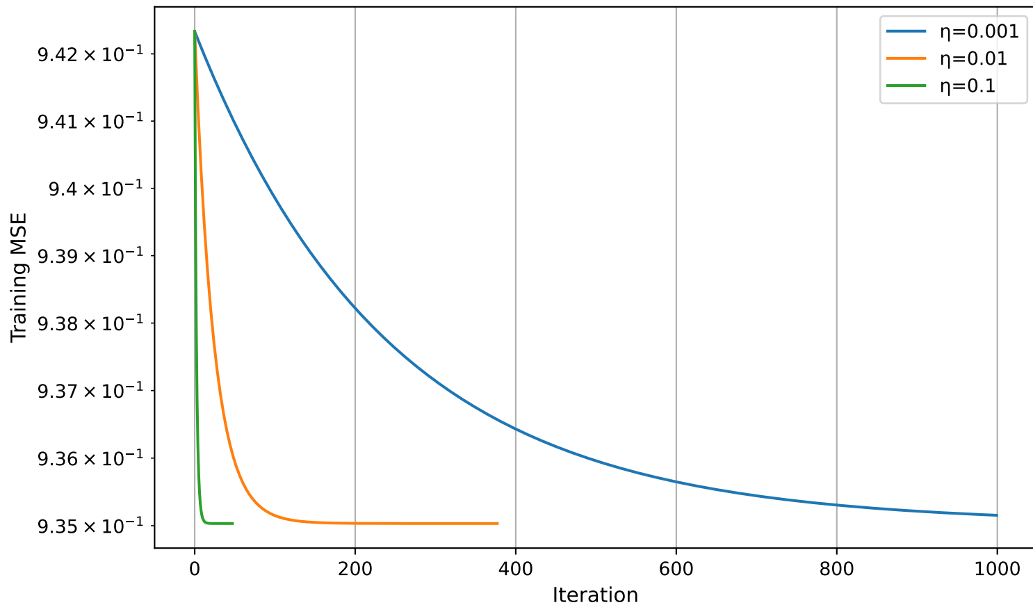
GD Training MSE vs Iteration (N=1000, p=10, seed=42)
