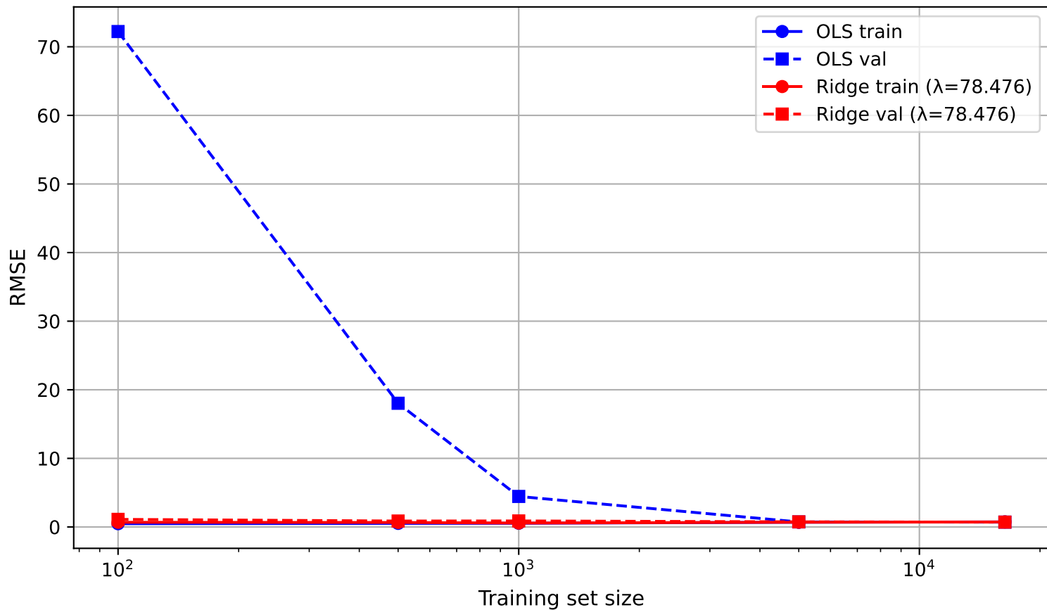
Learning Curves: OLS vs Ridge (California Housing)
