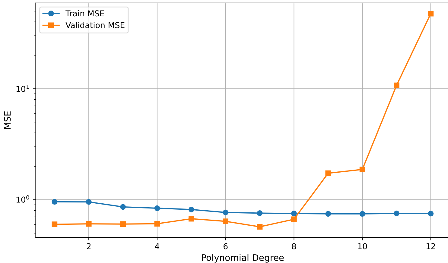
Polynomial Fitting: Train vs Validation MSE (California Housing, MedInc)
