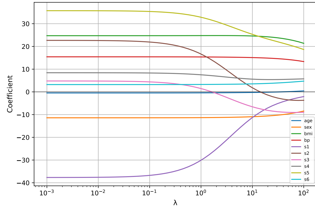
Ridge Coefficient Paths (Diabetes, standardized)
