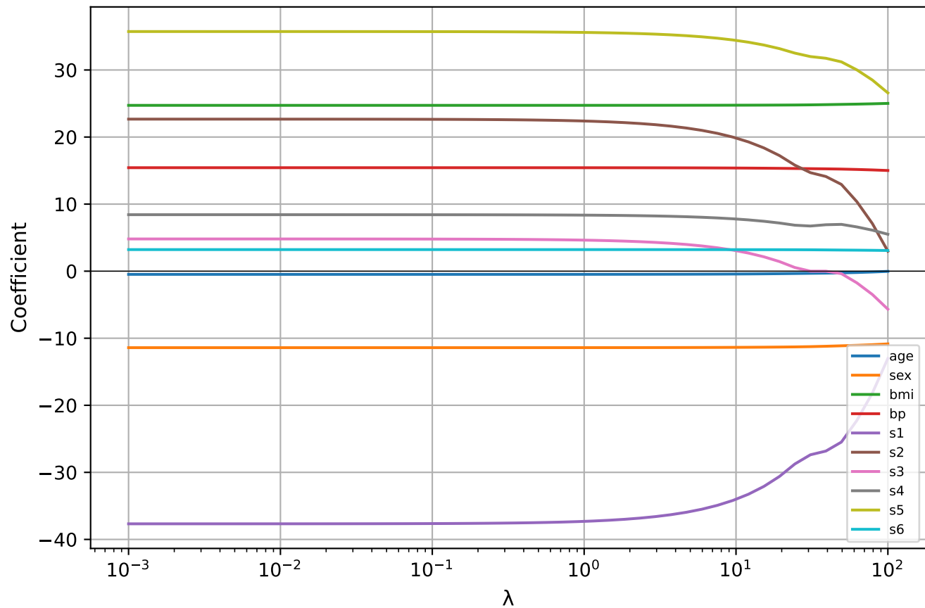
Lasso Coefficient Paths (Diabetes, standardized)
