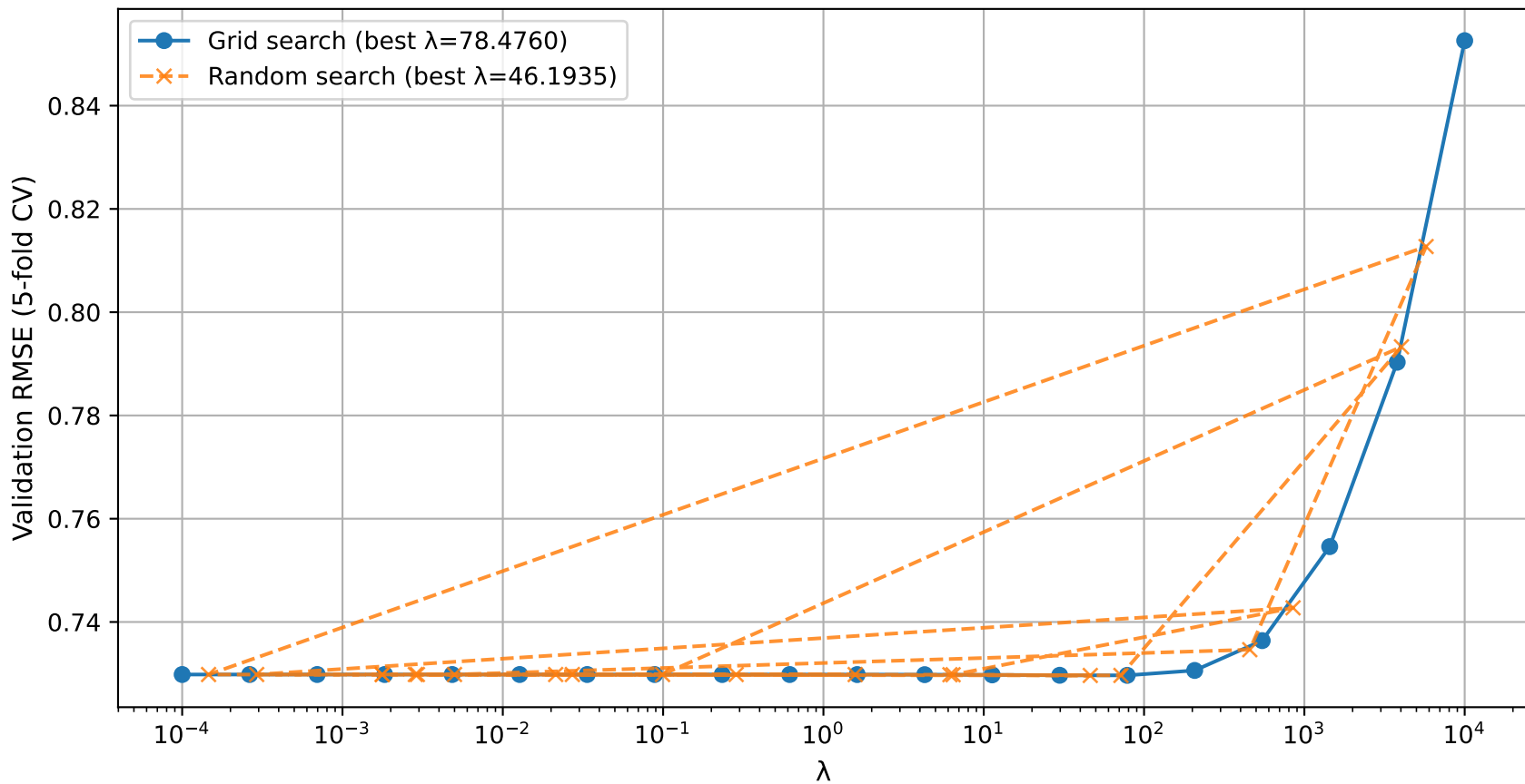
Ridge Hyperparameter Search: Grid vs Random (California Housing)
