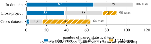
(b) all 260 comparisons, grouped by how the encoder was tested
