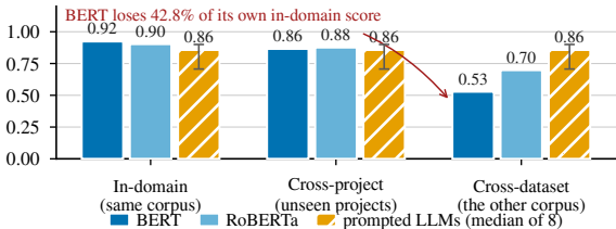
(a) security task on PROMISE_exp: the same 968 items scored at each level of distribution shift
