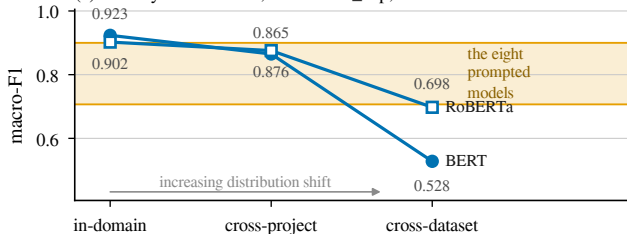
(b) all 260 paired encoder-vs-LLM comparisons
