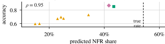
(b) the 8 prompted models, FR/NFR: accuracy tracks how far the predicted class share sits from the true one
