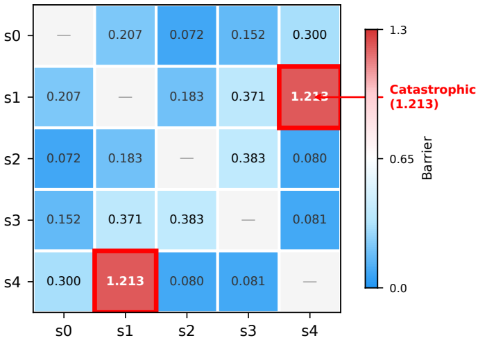
A Medical high-div seed-pair barrier matrix
