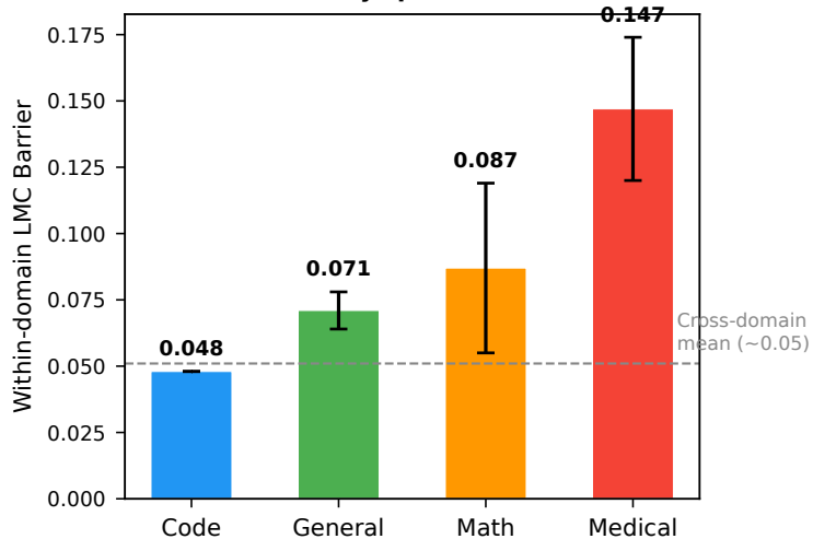
B Domain stability spectrum
