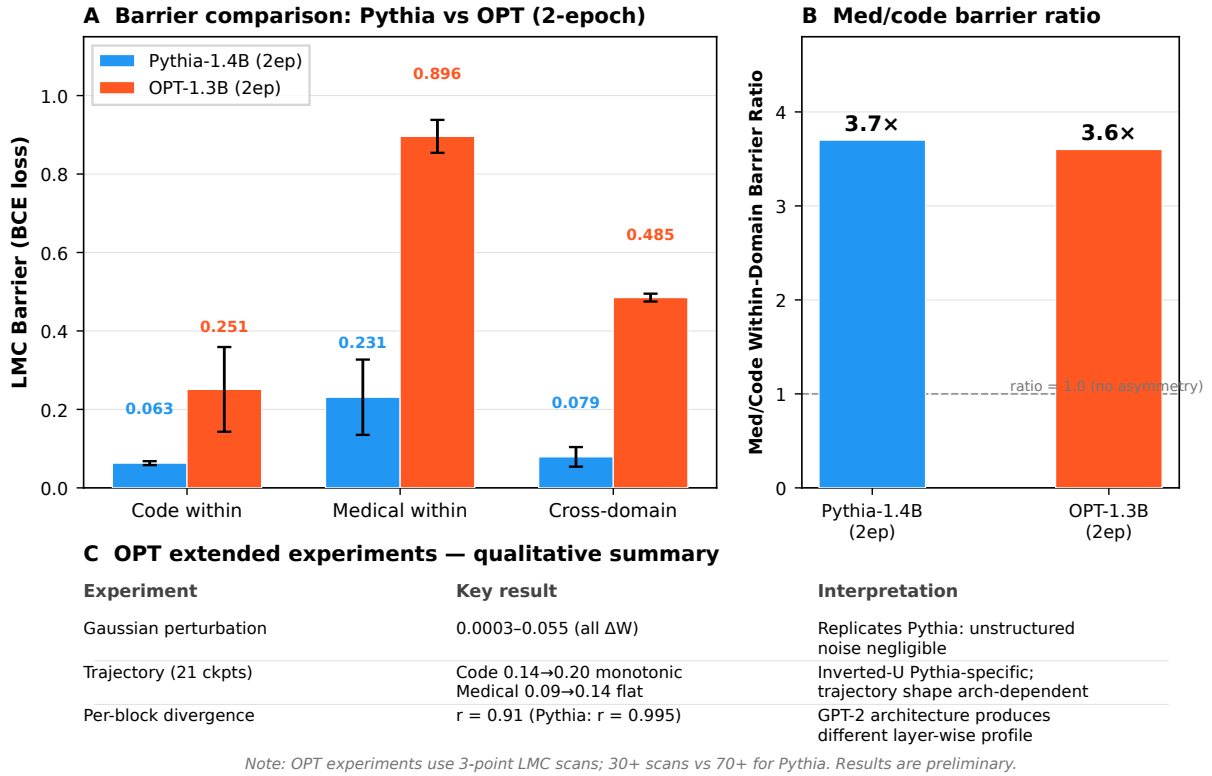
Figure 4: Cross-architecture replication on OPT-1.3B. Panel A: Barrier comparison between Pythia-1.4B and OPT-1.3B at 2-epoch training — code within, medical within, and cross-domain. Error bars show \pm 1\sigma . Panel B: Med/code within-domain barrier ratio — remarkably consistent at 3.7\times (Pythia) and 3.6\times (OPT), confirming the domain stability gradient generalizes across architectures. Panel C: Qualitative summary of OPT extended experiments (Gaussian perturbation, training trajectory, per-block divergence). See text for details.
