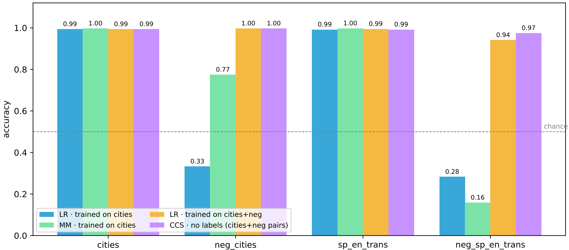
Negation moves statements off the training manifold — adding neg pairs (or dropping labels) fixes it
