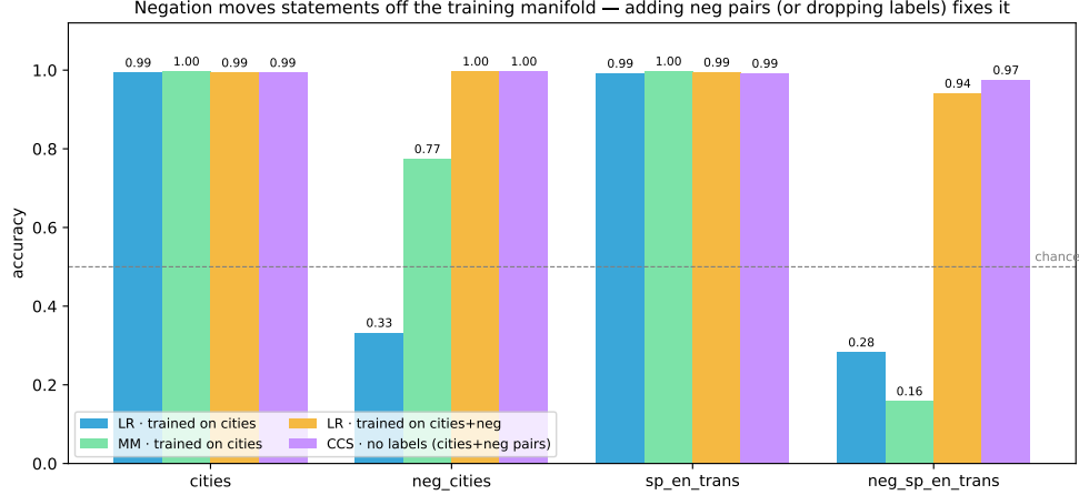
Figure 5: The transfer failures live on negated statements. Probes trained on affirmative statements alone (blue/green) collapse exactly on the negated variants; adding negated counterparts to training (orange) repairs it, and the label-free CCS probe (purple) repairs it without ever seeing a label . Same LLaMA-2-13B layer-14 protocol as Fig. 3.
