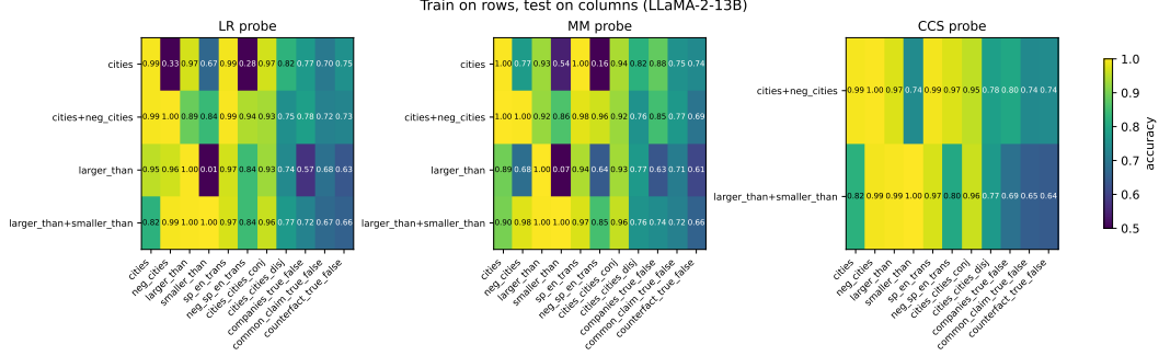
Figure 3: Do truth probes generalize? Each row trains on one (combination of) dataset(s); each column tests on another. Reproduces the Fig. 5 analysis of Marks and Tegmark [2024].
