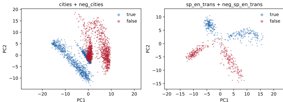
LLaMA-2-13B layer 14: last-token activations, top 2 PCs
