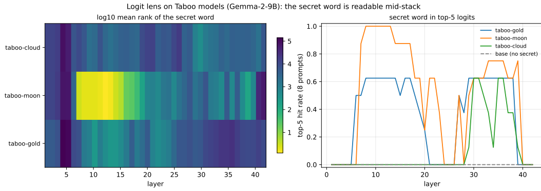
Figure 7: Where the secret lives. Left: \log_{10} mean rank of the secret word at each layer (brighter = more readable). Right: fraction of the eight hint prompts for which the secret word is in the layer’s top-5 logits. The base model control (dashed) never contains the signal. Our reproduction of the logit-lens analysis of Cywiński et al. [2025].
