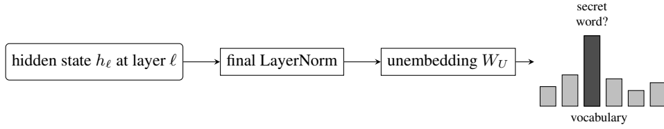
Figure 6: Logit lens. Decoding an intermediate hidden state with the model’s own final layer norm and unembedding reveals which tokens the layer “prefers”. For Taboo models, the secret word rises to the top ranks at middle layers even though the output never contains it.
