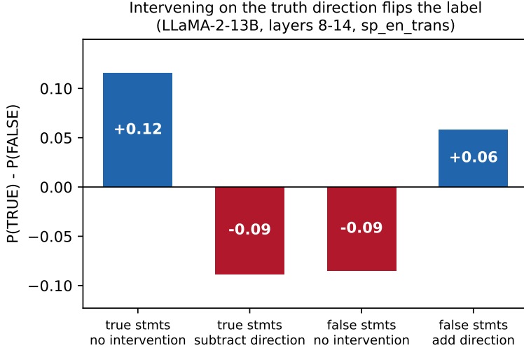
Figure 5: The probe direction is causally used. Adding the MM truth direction to the residual stream (layers 8–14) moves P(\text{TRUE}) - P(\text{FALSE}) for false statements from negative to positive; subtracting it does the reverse for true statements (177 sp_en_trans statements per condition, few-shot TRUE/FALSE prompt). Compare Table 2 of Marks and Tegmark [2024].
