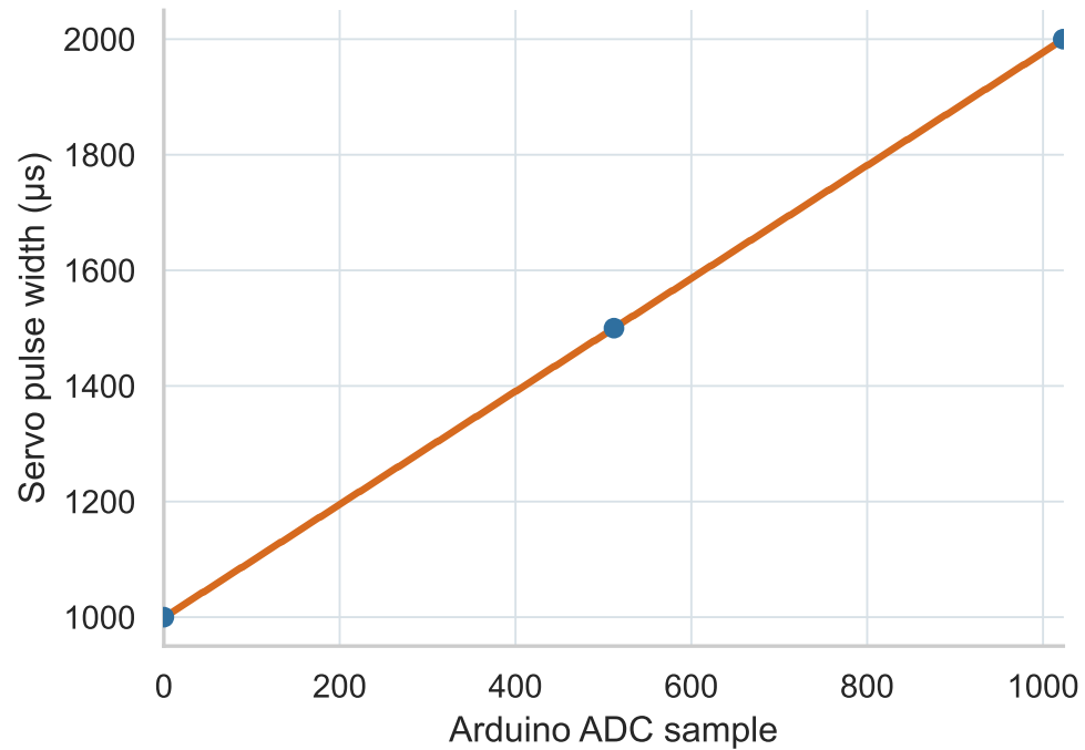
Task 4: linear servo command mapping
