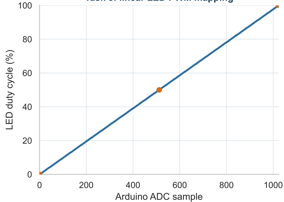
Task 3: linear LED PWM mapping
