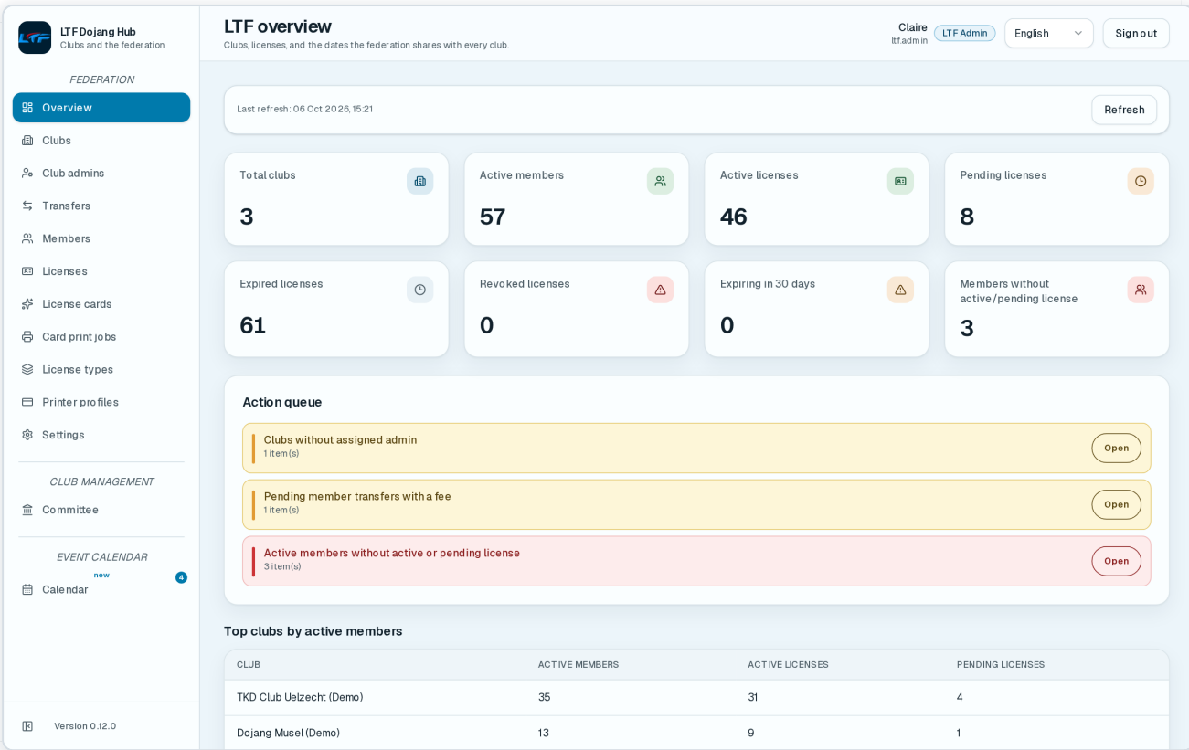
Figure 40 · The LTF overview
