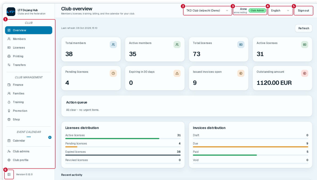
Figure 3 · The club overview with the main parts of the screen
