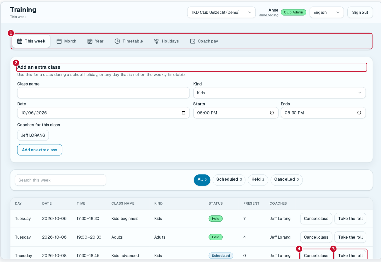
Figure 25 · The training week
