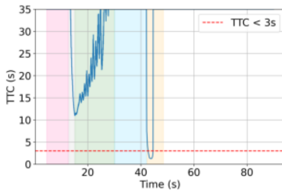
Time To Collision (TTC)
