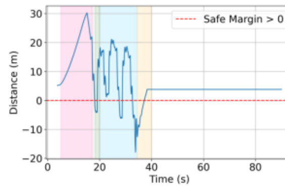
RSS Safety Margin
