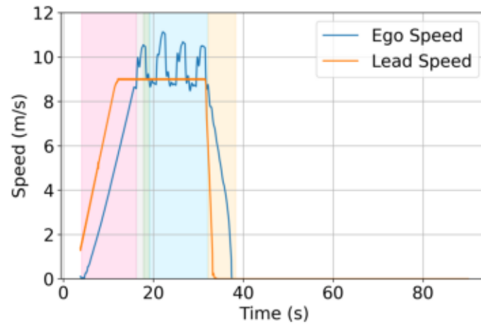
Ego and Lead Vehicle Speed
