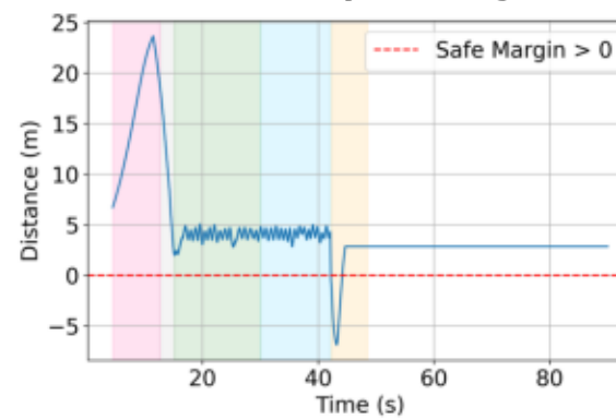
RSS Safety Margin
